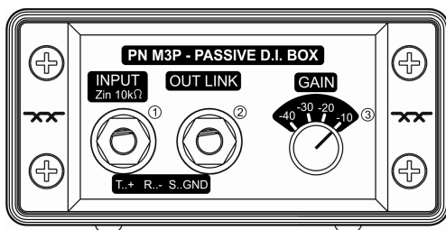
FIG. 1 - Painel Frontal
